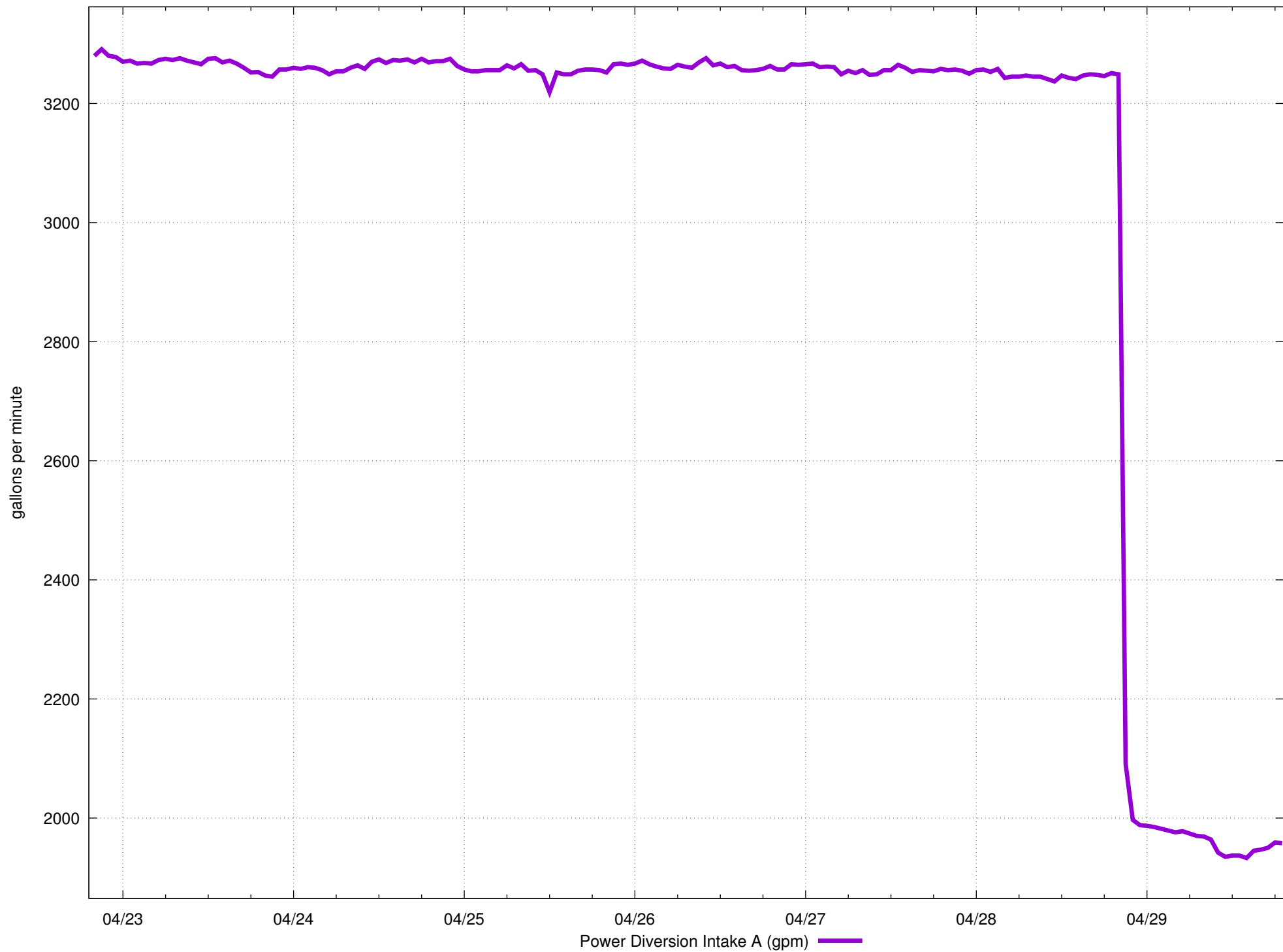
Power Diversion
