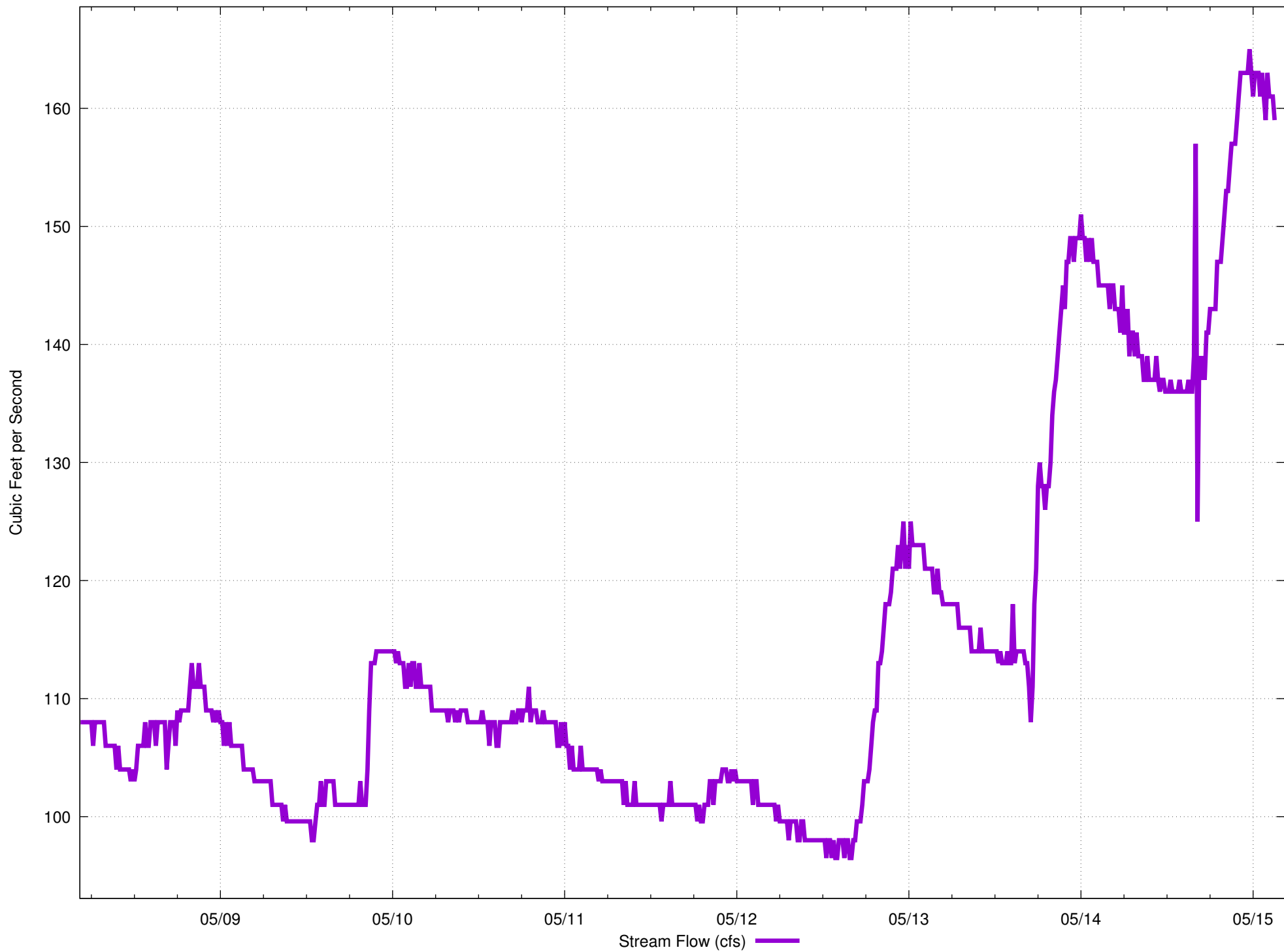
Beaver River near Beaver, Utah (USGS)
