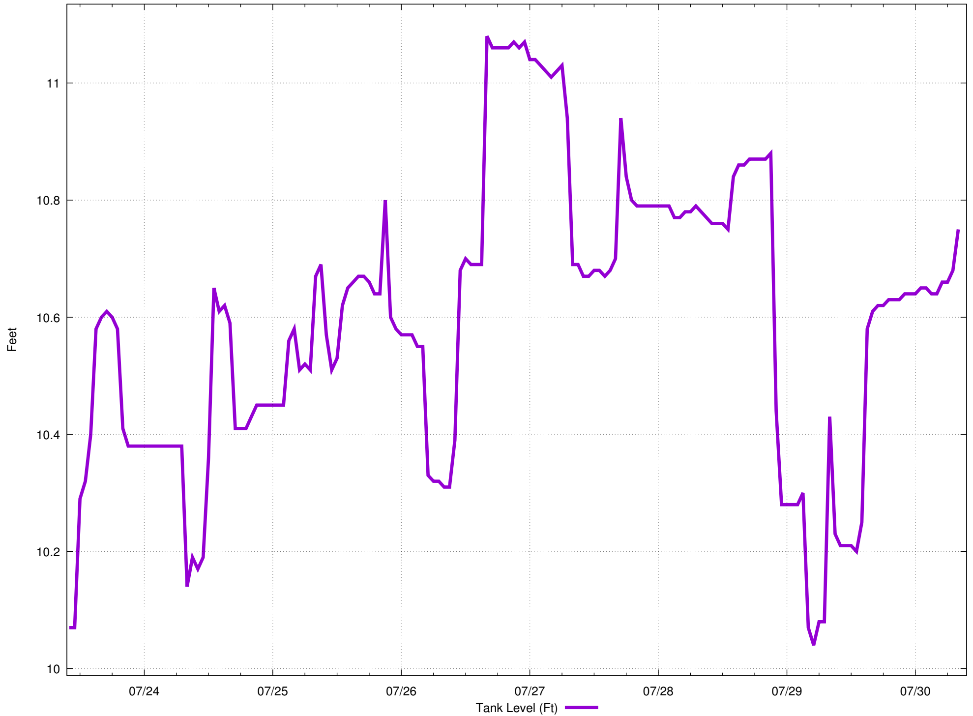
Surge Tank
