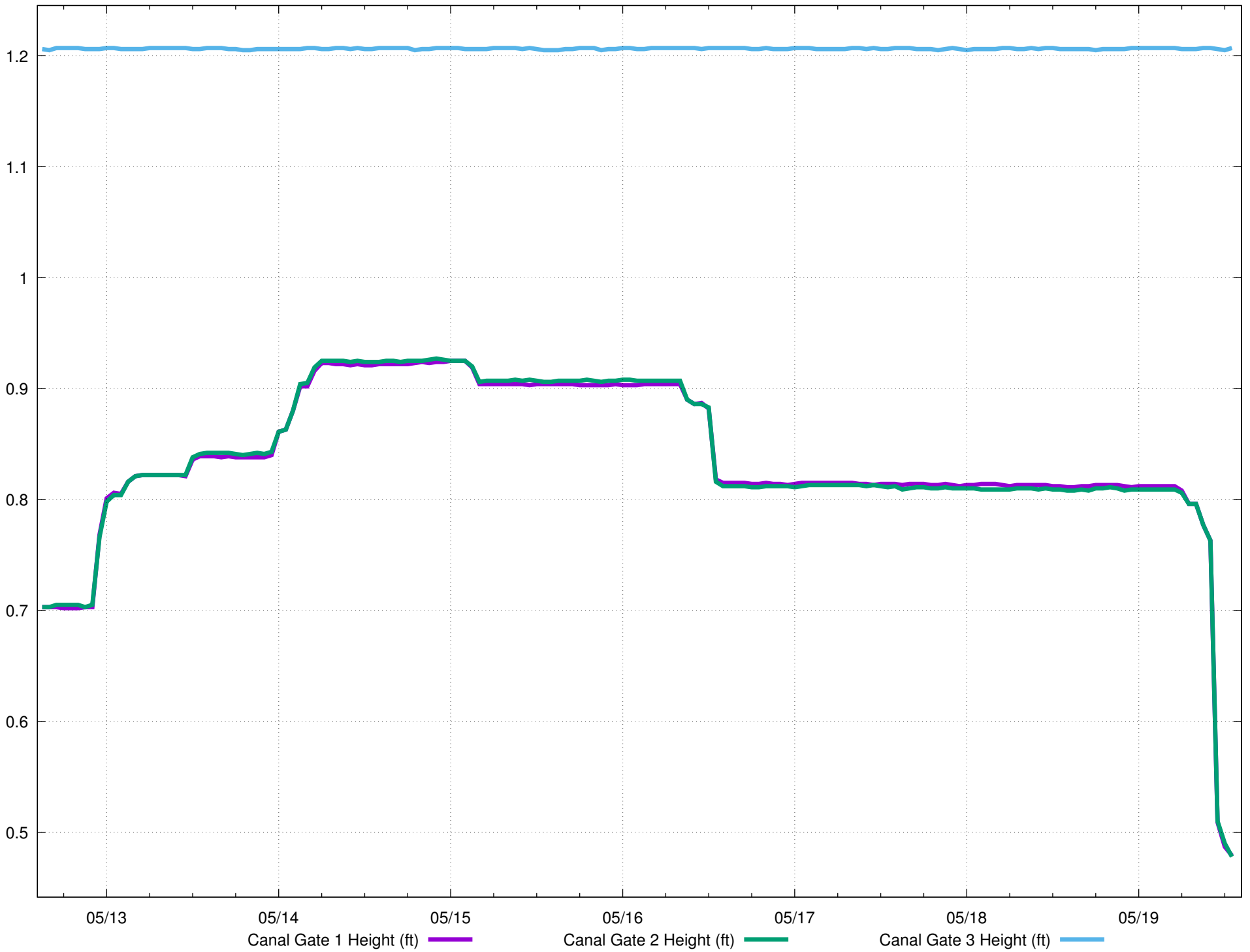
Richfield Canal Gate Heights
